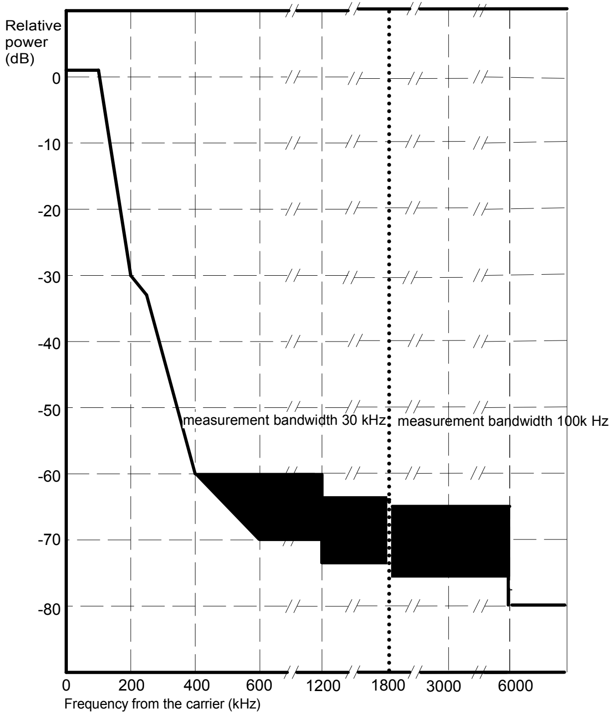
Figure A.2a: GSM 400, GSM 900, GSM 850, GPRS 850, DCS 1800, PCS 1900 and GPRS 1900 BTS spectrum due to GMSK modulation
